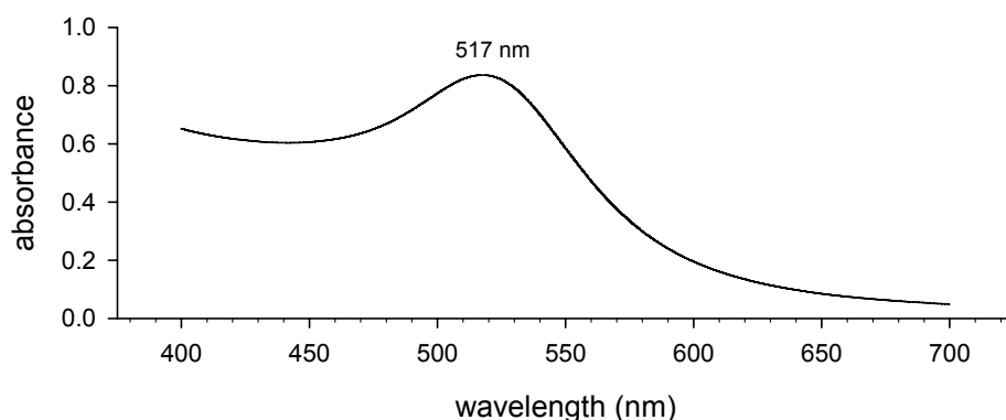
Figure 1. Representative optical absorbance spectrum for the native suspension, centered on the surface plasmon resonance peak for Au. Wavelength at peak maximum is indicated.
