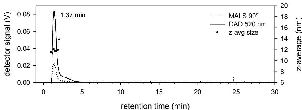
Figure 2. Representative AFFF retention trace showing detector response for 90^\circ light scattering and 520 nm optical absorption. The z-average hydrodynamic diameter values are given across the peak trace. A secondary feature (hump) centered at 3 min indicates the presence of detectable clusters (e.g., dimers, trimers) or larger Au monomers at concentrations too low to quantify by DLS.
