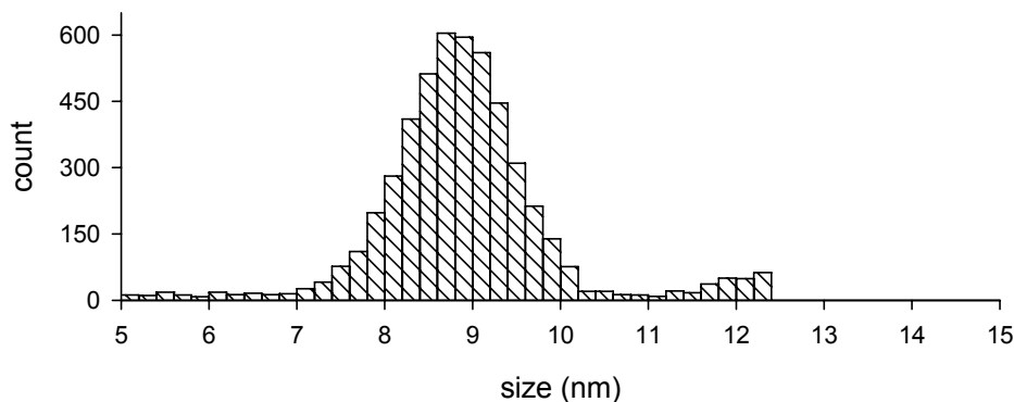
Figure 6. Particle size histogram generated by TEM analysis.
