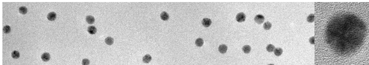
Figure 3. TEM micrographs. On left: image of Au particles sampled from a single representative TEM image. On right: high magnification TEM image revealing internal structure and faceting of a single Au particle.
